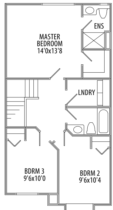
SECOND FLOOR 702 SQ.FT.
