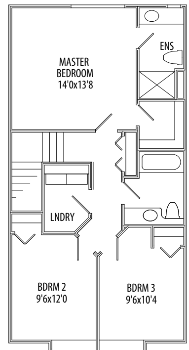
SECOND FLOOR 718 SQ.FT.
